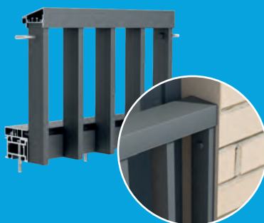
JULIET BALCONY SYSTEMS INNER MOUNTED OPTION
